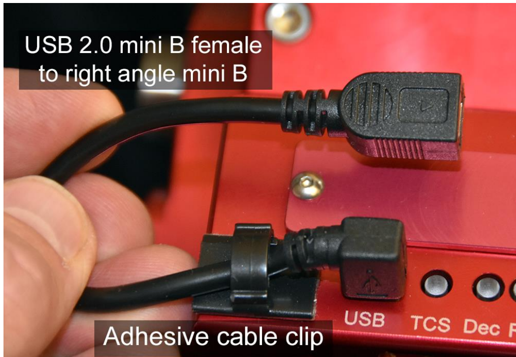
Figure 1: The right-angle mini-B connector plugged into the USB Port is captivated by the adhesive cable clip.
